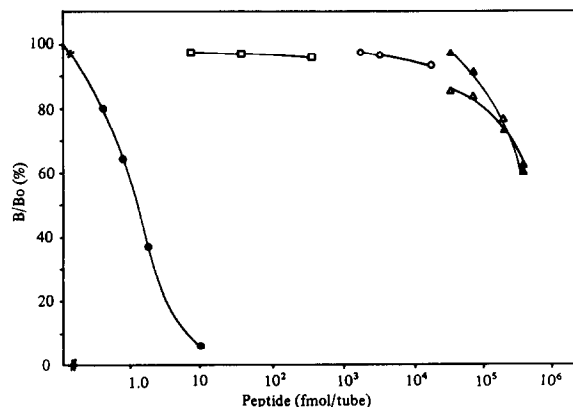
Fig.2. Crossreactivities of ANP and related peptides in BNP RIA. Serial dilution curves of pBNP(1-26) (●), \alpha -hANP (Δ), \beta -hANP (○), \gamma -hANP (□), and \alpha -rat ANP (▲) are shown.
